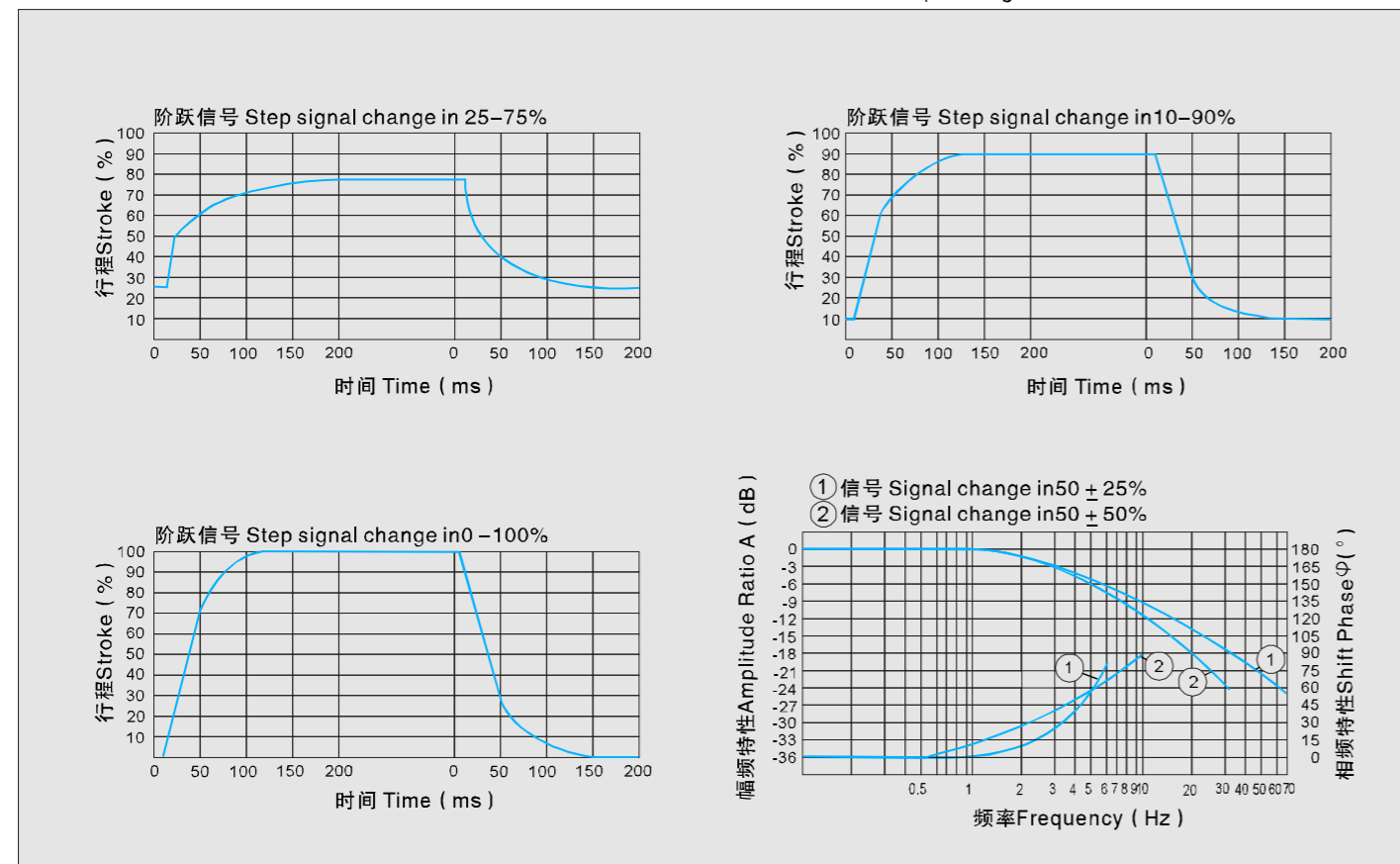
02型特性曲线 (试验条件 v=36 \times 10^{-6} \text{m}^2/\text{S} t=50^\circ\text{C} ) Model Characteristic Curves (Testing Condition v=36 \times 10^{-6} \text{m}^2/\text{S} t=50^\circ\text{C} )
