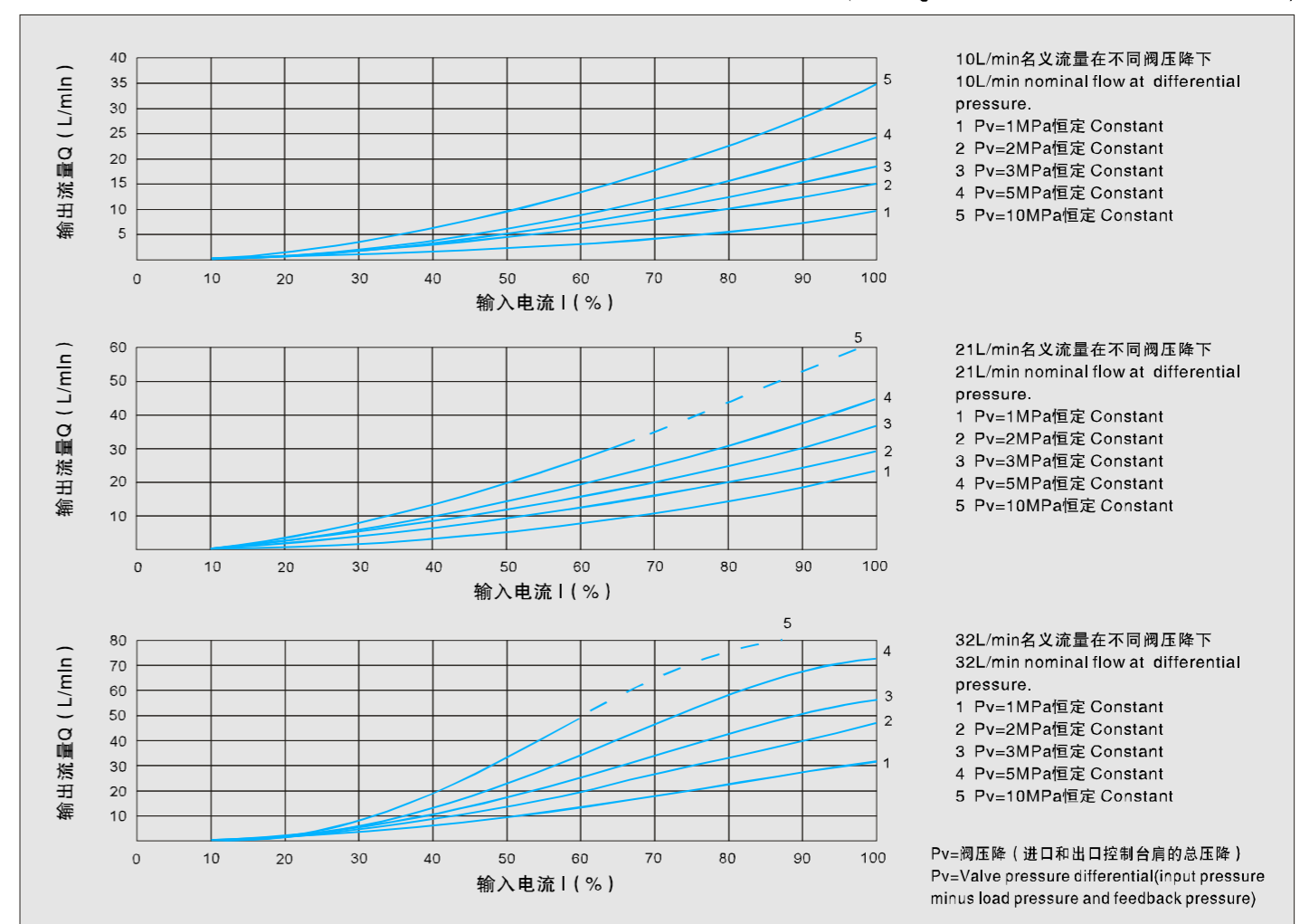
03型特性曲线 (试验条件 v=36 \times 10^{-6} \text{m}^2/\text{S} t=50^\circ\text{C} ) 03Model Characteristic Curves (Testing Condition v=36 \times 10^{-6} \text{m}^2/\text{S} t=50^\circ\text{C} )
