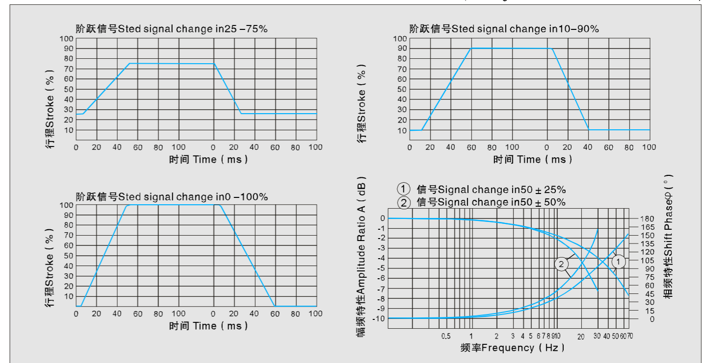
03型特性曲线 (试验条件 v=36 \times 10^{-6} \text{m}^2/\text{S} t=50^\circ\text{C} ) 03Model Characteristic Curves (Testing Condition v=36 \times 10^{-6} \text{m}^2/\text{S} t=50^\circ\text{C} )
